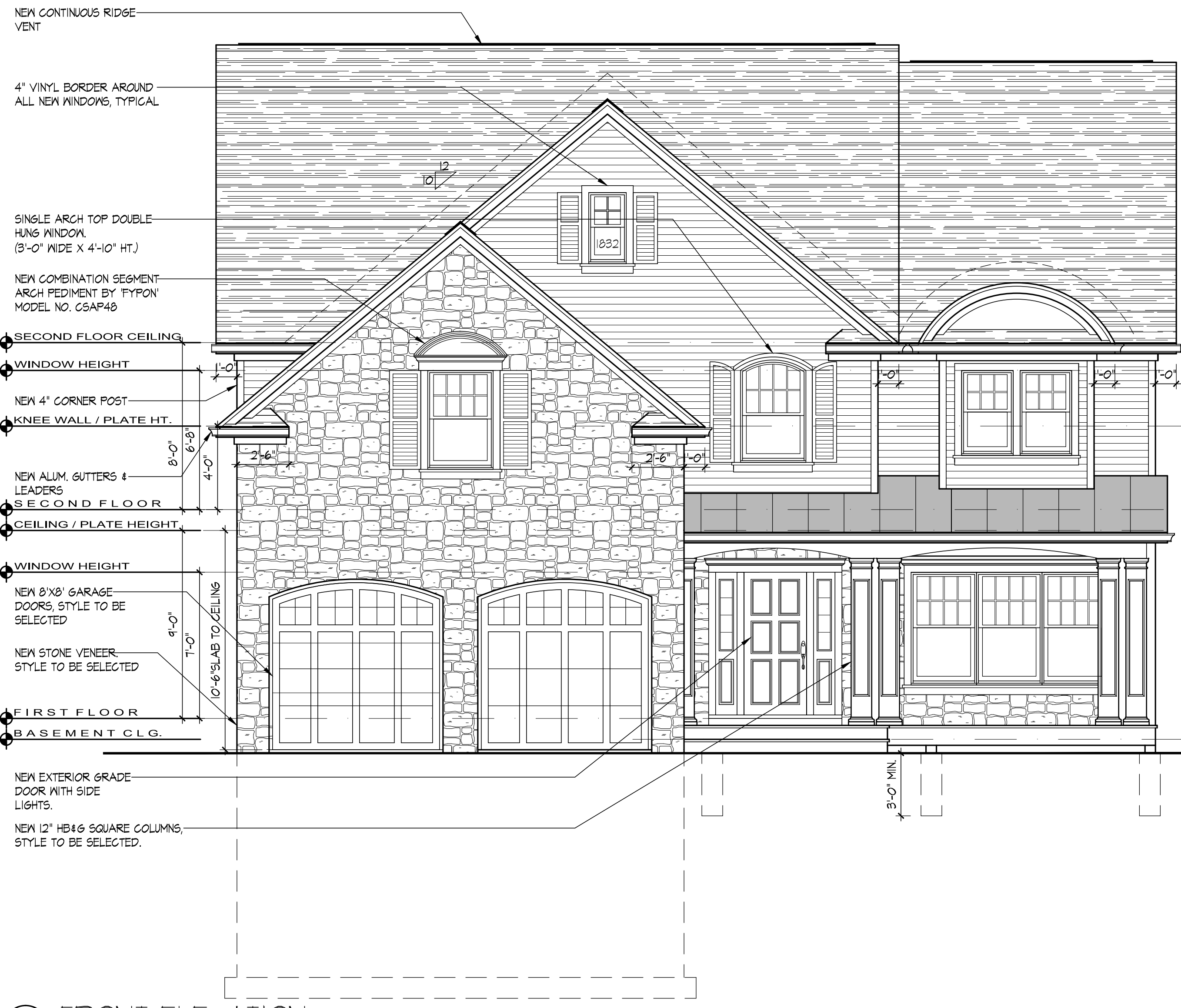
1 FRONT ELEVATION SCALE: 1/4" = 1'-0"
